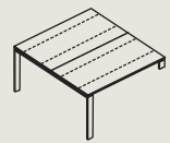
EVB 19/20/21-4 140/160/180x140x75h
